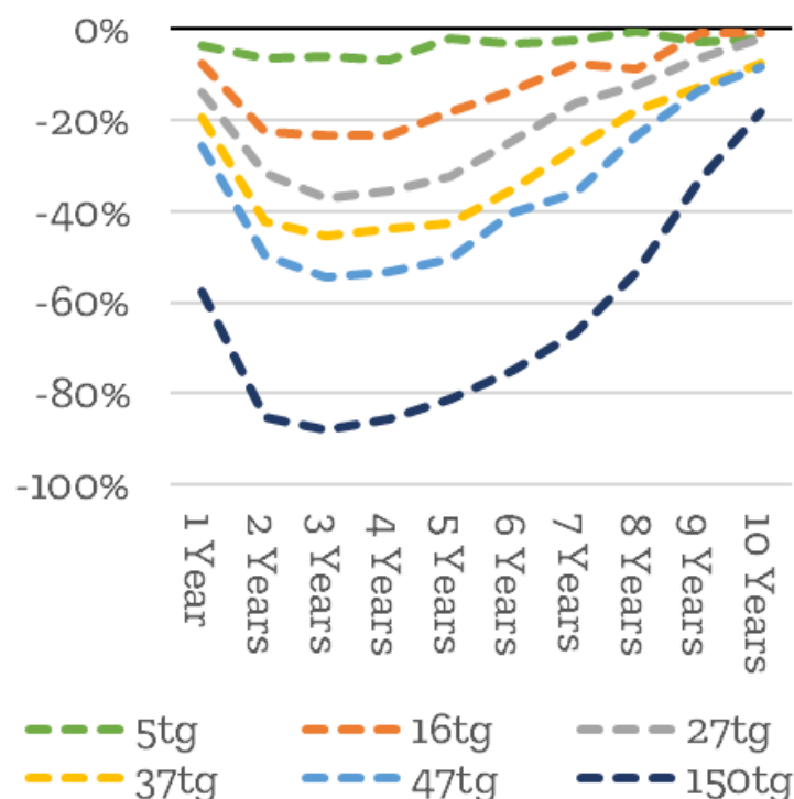
Figure 1. Decrease in global heat production if there were no response measures, estimates over time at different magnitudes of nuclear winter (Xia et al., 2022).
